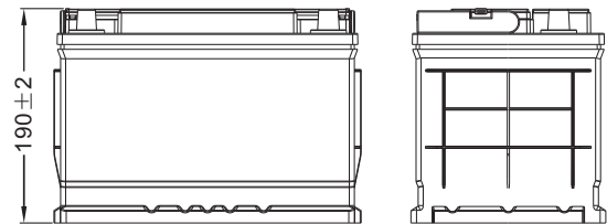
Dimensions (mm)
